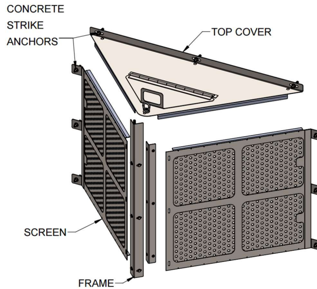
V-CONFIGURATION
