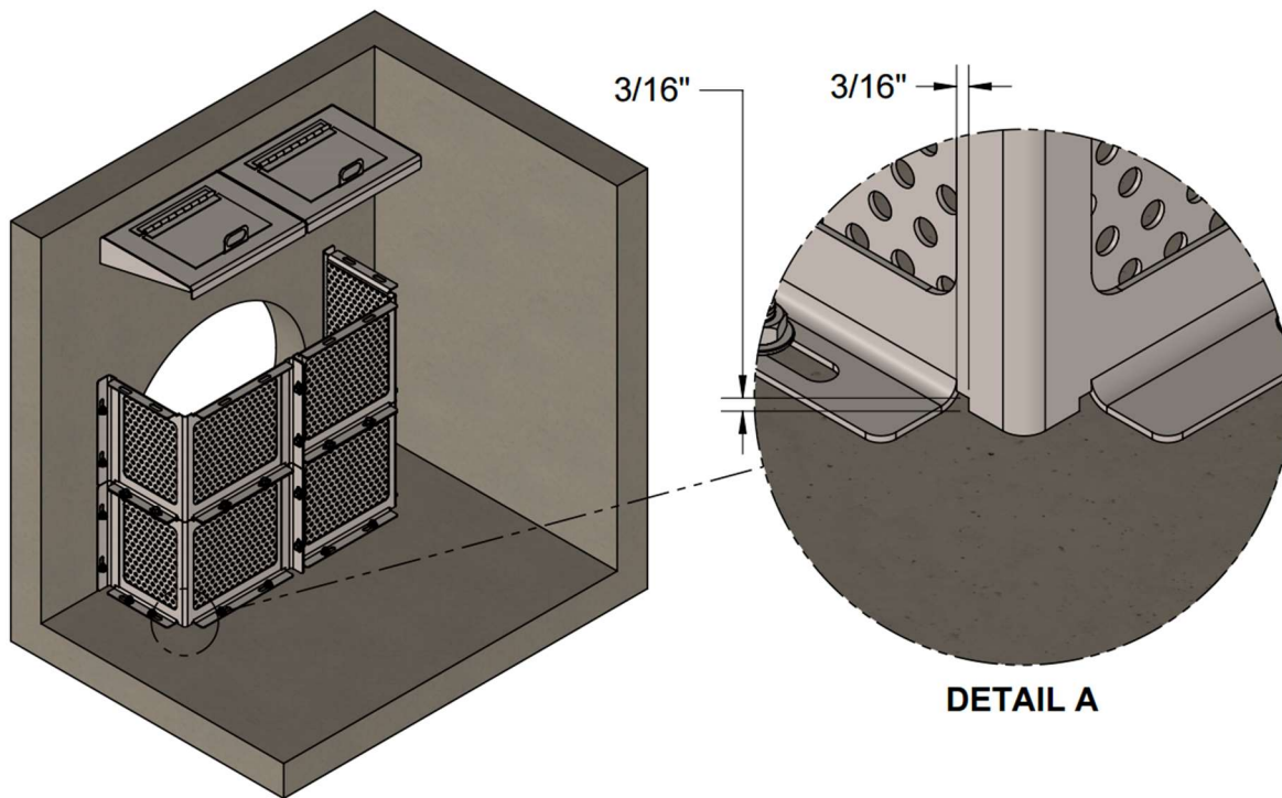
SEEPAGE HOLES
