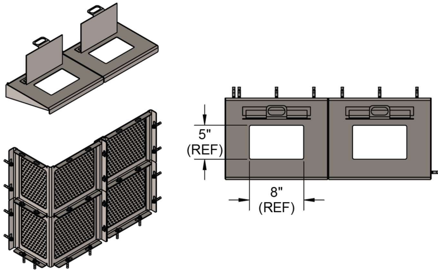
L-CONFIGURATION
